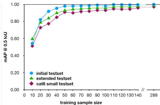
Variation of the mAP @0.5 IoU on three different test sets based on the number of OPTs used for training the object detector.
