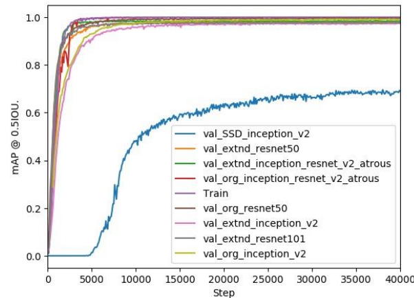
Difference of the mAP @0.5 IoU on a validation set for different SSD and Faster-RCNN based models.
