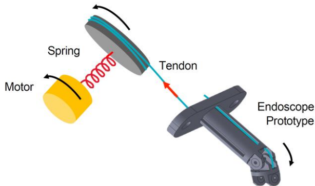
Series elastic actuation is a concept where a spring is placed in a mechanical system between the motor and the moving part, in this case the tendon-driven endoscope. (Image: Sara Pensotti)
